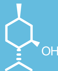
Chemical structure of L-Menthol
